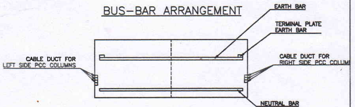
SECTION - "A-A"
