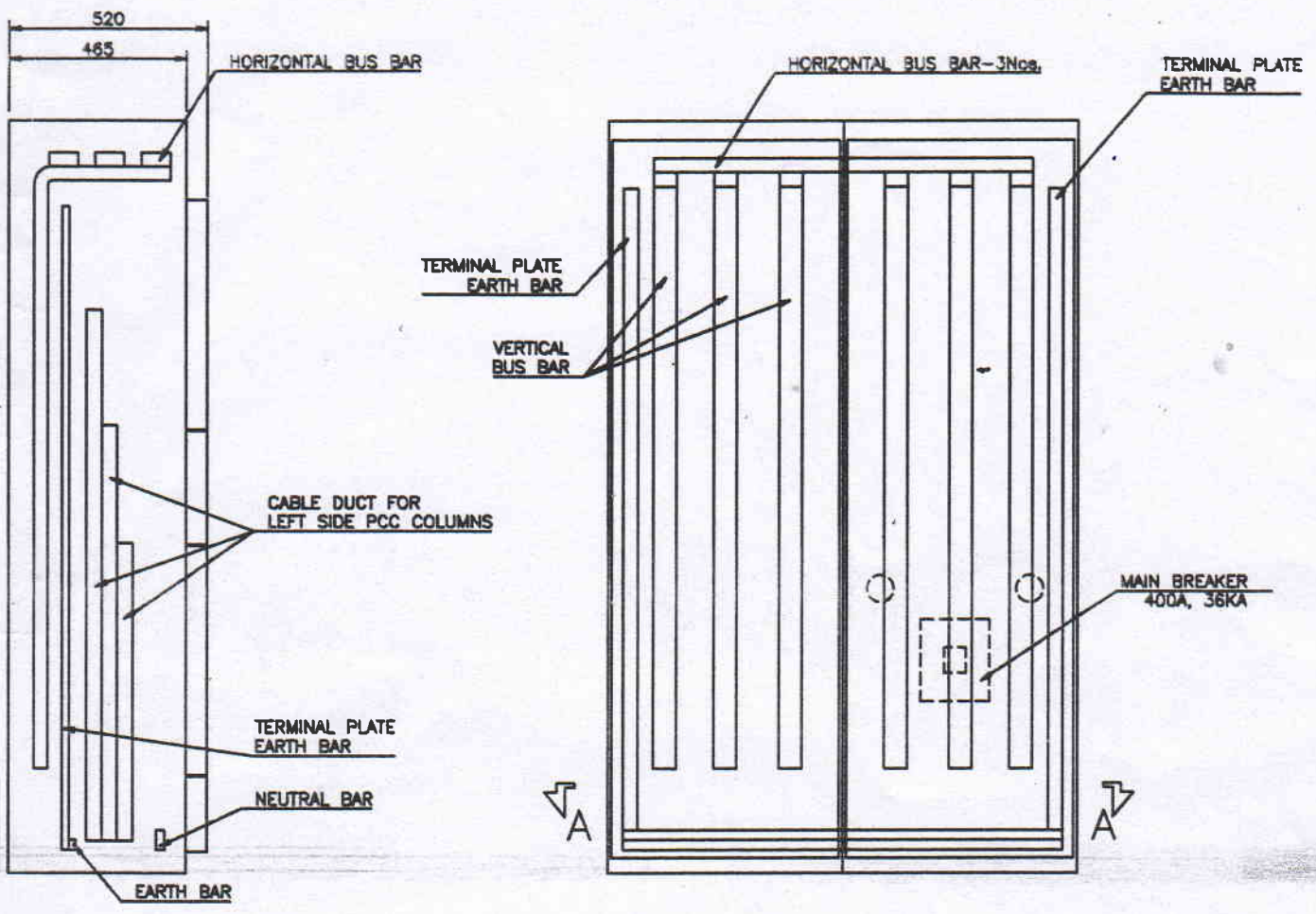
BUS-BAR ARRANGEMENT
