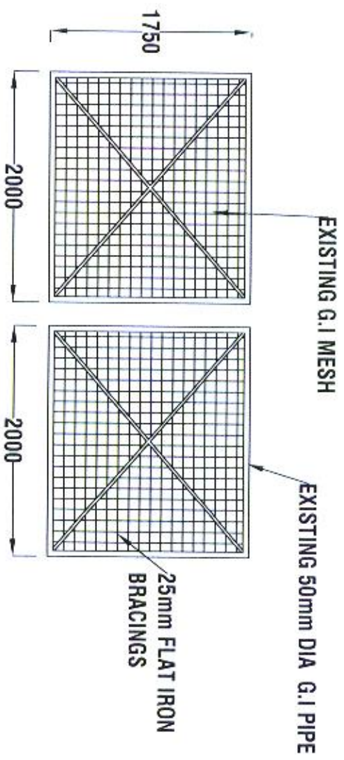
EXISTING STEEL GATE
